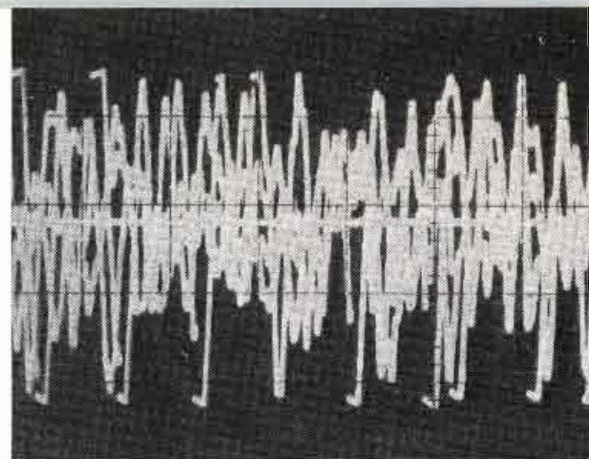
Figure 2. Taking a look at what the transmitter sees coming out of the limiter. It is necessary to preemphasize the FM limiter output to simulate the stereo generator's preemphasis to properly observe the transmitter's modulation input. Even though clipping may not be visible at the limiter output because of internal deemphasis, this method of testing will reconstruct the waveforms and show you what the transmitter sees. The photo shows peak clipping by the safety clippers in an FM limiter during a heavily scored passage. These pulse-like inputs can result in ringing in stereo generator filter circuits. More moderate input levels to the limiter resulted in negligible clipping.
